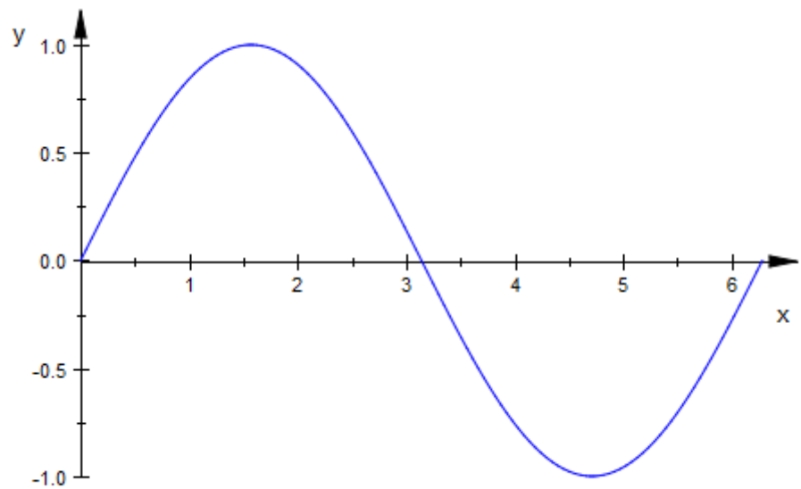
the sine function
